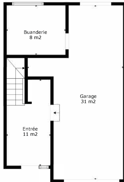
Rez
