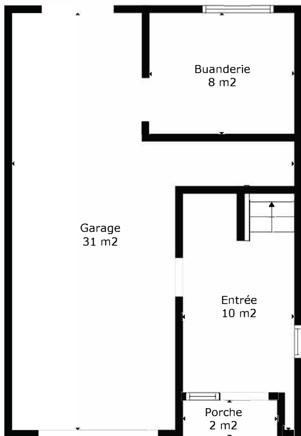
Rez
