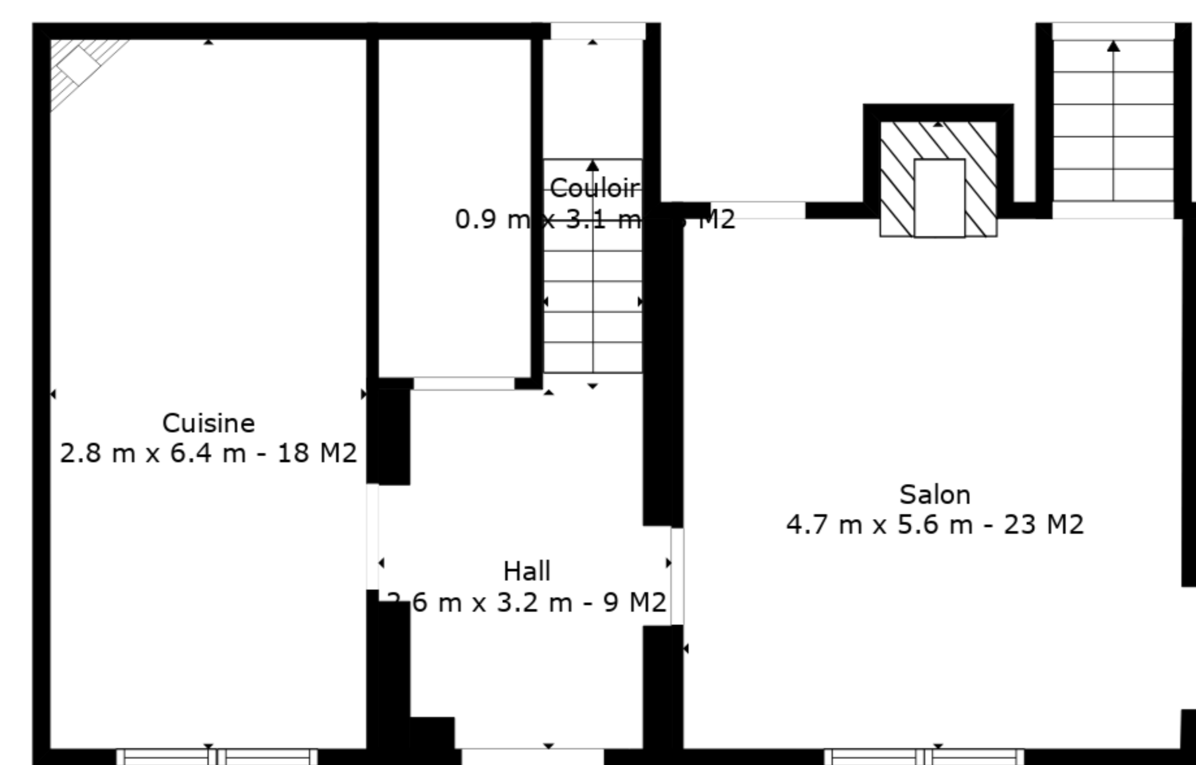
Rez
